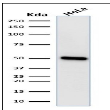
Fig. 3: Western Blot Analysis of human HeLa cell lysate using FOXA1 Monoclonal Antibody (FOXA1/1518).
