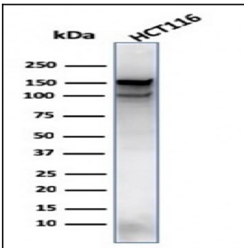
Fig. 3: Western Blot Analysis of HCT116 cell lysate using MSH6 Mouse Monoclonal Antibody (MSH6/3089).
