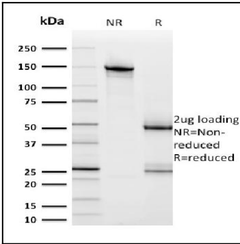
Fig. 2: SDS-PAGE Analysis HER-2 Mouse Monoclonal Antibody (ERBB2/2453). Confirmation of Purity and Integrity of Antibody.
