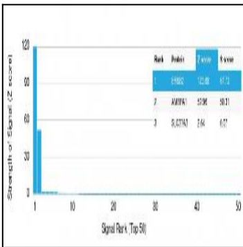
Fig. 3: Analysis of Protein Array containing more than 19,000 full-length human proteins using HER-2 Mouse Monoclonal Antibody (ERBB2/2453). Z- and S- Score: The Z-score represents the strength of a signal that a monoclonal antibody (Monoclonal Antibody) (in combination with a fluorescently-tagged anti-IgG secondary antibody) produces when binding to a particular protein on the HuProt™ array. Z-scores are described in units of standard deviations (SD's) above the mean value of all signals generated on that array. If targets on HuProt™ are arranged in descending order of the Z-score, the S-score is the difference (also in units of SD's) between the Z-score. S-score therefore represents the relative target specificity of a Monoclonal Antibody to its intended target. A Monoclonal Antibody is considered to specific to its intended target, if the Monoclonal Antibody has an S-score of at least 2.5. For example, if a Monoclonal Antibody binds to protein X with a Z-score of 43 and to protein Y with a Z-score of 14, then the S-score for the binding of that Monoclonal Antibody to protein X is equal to 29.
