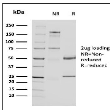
Fig.1: SDS-PAGE Analysis Purified Uroplakin 1A Mouse Monoclonal Antibody (UPK1A/2924). Confirmation of Purity and Integrity of Antibody.
