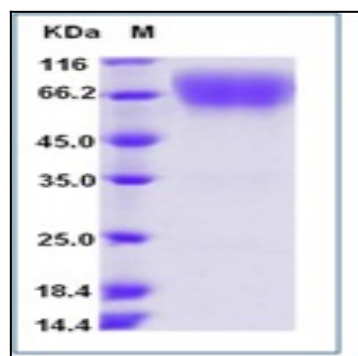
Fig 1: Mouse CD86 / B7-2 Recombinant Protein (Fc Tag)
