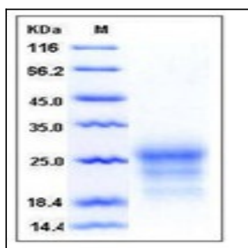
Fig 1: Mouse CD90 / THY-1 Recombinant Protein (His Tag)
