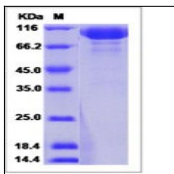
Fig 1: Human Pregnancy Specific GlycoRecombinant Protein 1 Recombinant Protein (Fc Tag)
