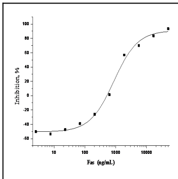
Fig 2: Human FAS / CD95 / APO-1 / TNFRSF6 Recombinant Protein (His Tag) measured by its ability to inhibit Fas Ligand induced apoptosis of Jurkat human acute T cell leukemia cells.
