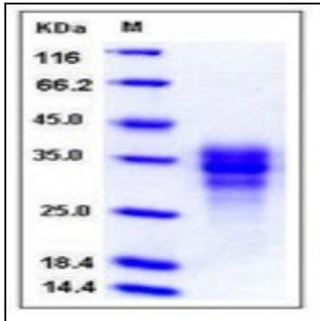
Fig 1: Human FAS / CD95 / APO-1 / TNFRSF6 Recombinant Protein (His Tag)
