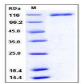
Fig 1: Human VCAM-1 / CD106 Recombinant Protein (His Tag)
