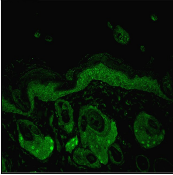
Figure1 : Mouse Anti-Hsp70 Antibody [N27F3-4] used in Immunohistochemistry (IHC) on Mouse backskin
