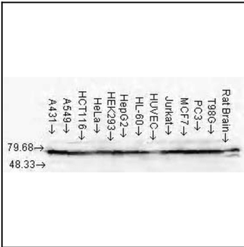
Figure 2 : Mouse Anti-Hsp70 Antibody [N27F3-4] used in Western Blot (WB) on Human Cell lysates
