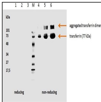
Figure-1: Human transferrin detected by the mouse monoclonal antibody HTF-14. 1. hTransferrin; 5 \mu g/well (red. con.) 2. hTransferrin; 3 \mu g/well (red. con.) 3. hTransferrin; 1 \mu g/well (red. con.) M. Low Range marker (Bio-Rad) 4. hTransferrin; 1 \mu g/well (non-red. con.) 5. hTransferrin; 3 \mu g/well (non-red. con.) 6. hTransferrin; 5 \mu g/well (non-red. con.)
