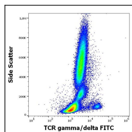
Figure 2: Flow cytometry surface staining pattern of human peripheral whole blood stained using anti-human TCR gamma/delta (B1) FITC antibody
