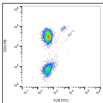
Figure 1: Surface staining of human peripheral blood lymphocytes with anti-human TCR gamma/delta (B1) FITC.
