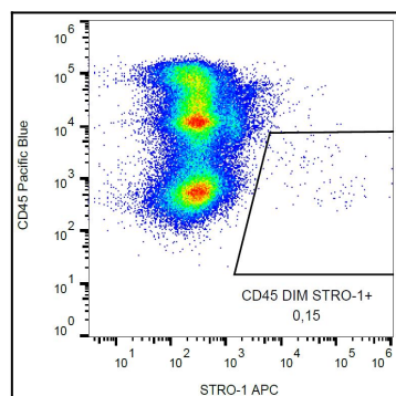
Figure 1: Surface staining of human peripheral blood with anti-STRO-1 (STRO-1) APC.
