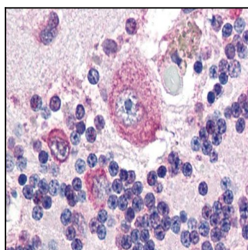
Figure 1: Immunohistochemistry staining of human cerebellum (paraffin sections) using anti-PLAP (H7E8).
