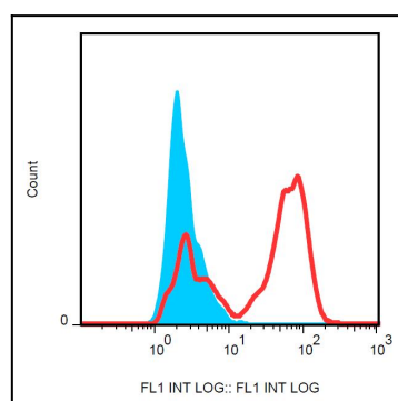
Figure 1: Surface staining of HLA-G transfectants with anti-HLA-G antibody (87G) FITC.
