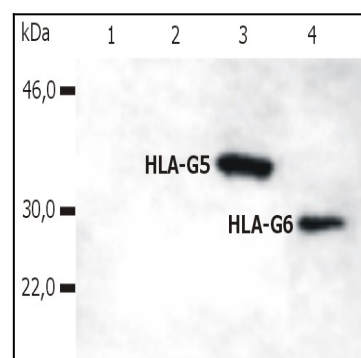
Figure 1: Western Blotting analysis of whole cell lysate of HLA-G stable transfectants (various splice variants) using anti-human HLA-G (5A6G7). Lane 1: M8 cell line transfected with empty vector. Lane 2: M8 cell line transfected with HLA-G1. Lane 3: M8 cell line transfected with HLA-G5. Lane 4: M8 cell line transfected with HLA-G6
