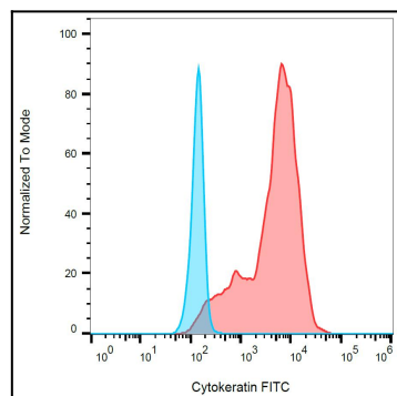
Figure 1: Intracellular flow cytometry analysis of cytokeratin expression in HeLa cells using anti-cytokeratin antibody (C-11) FITC.
