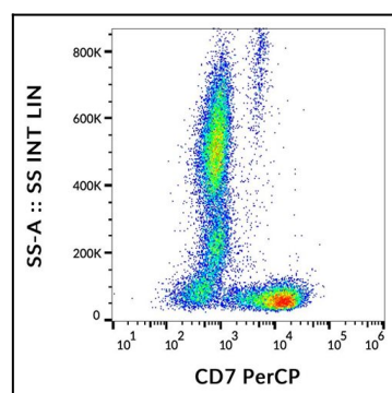
Figure 1: Flow Cytometry of PBMC with anti- h CD7 PerCP
