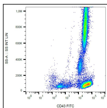
Figure 1: Surface staining of human peripheral blood with anti-CD43 (MEM-59) FITC.
