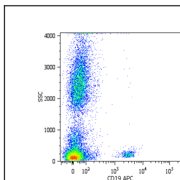
Figure 1: Surface staining of human peripheral blood cells with anti-human CD19 (LT19) APC.
