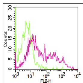
Fig.1: Cell surface staining of PBMC (lymphocytes gated). Green Isotope control (Abeomics). Red: anti-HLADR (10-4181), clone AB3. 0.2 \mu g antibodies were used. Goat anti-mouse IgG PE (Abeomics) was used as secondary antibody.
