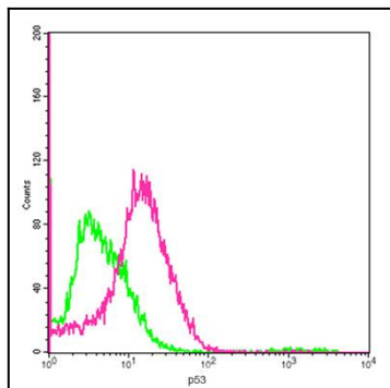
Figure-1 : Flow cytometric analysis of p53 Antibody (Clone: 6F2D3) on HEK293 at 2 \mu\text{g} for 1 \times 10^6 cells. Red histogram represents p53 Antibody (Clone: 6F2D3) and green histogram represents isotype control.
