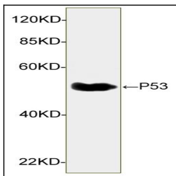
Figure-2 : Western blot analysis of p53 Antibody (Clone: 6F2D3) at 1 \mu\text{g}/\text{ml} on UV-treated HEK 293 cell lysates, IRDye 800 Conjugated Goat Anti-Mouse IgG was used as secondary Antibody.
