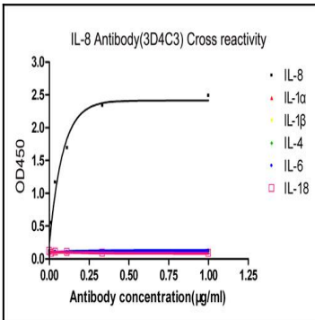
Figure-3 : ELISA analysis of Cross reactivity using IL-8 Antibody (Clone: 3D4C3).
