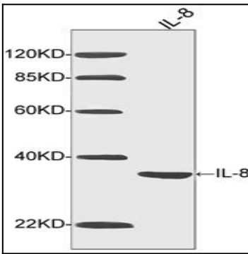
Figure-1 : Western blot analysis of IL-8 Antibody (Clone: 3D4C3) at 1 µg/ml on human recombinant IL-8 fusion protein, IRDye 800 Conjugated Goat Anti-Mouse IgG was used as secondary antibody.
