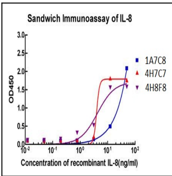
Figure-2 : Sandwich ELISA analysis of matched antibody pairs using IL-8 Antibody (Clone: 3D4C3) 1) ELISA plate was coated with Human IL-8 Antibody (3D4C3) 2) Human recombinant IL-8 protein at appropriate dilution was added into appropriate reaction wells 3) After a period of incubation, HRP conjugated Human IL-8 Antibody (Clone. 1A7C8, 4H7C7 and 4H8F8) was added by proper period of incubation.
