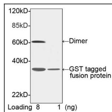
Figure-1 : Western blot analysis of Biotin conjugated GST-tag Antibody at 1 µg/ml on GST-tagged fusion protein (8 & 1 ng), The signal was developed with Streptavidin-HRP at 1:5,000 dilution.
