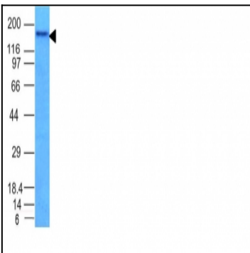
Western Blot Analysis of HCT116 Cell Lysate using CD56 Monoclonal Antibody (NCAM1/795)
