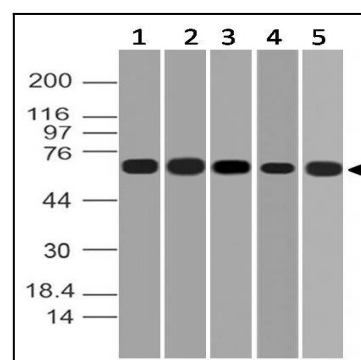
Figure-1: Western blot analysis of CNOT4. Anti-CNOT4 antibody (11-8113) was used at 2 µg/ml on (1) h Lung, (2) h Liver, (3) h Brain, (4) h Heart and (5) h Stomach lysates.
