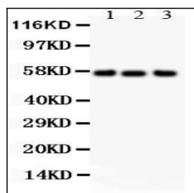
Figure 1: All Lanes: Anti ALPL(39-2015) at 0.5ug/ml. Lane 1: Human Placenta Tissue Lysate at 50ug, Lane 2: HT1080 Whole Cell Lysate at 40ug, Lane 3: JURKAT Whole Cell Lysate at 40ug. Predicted band size: 57 kDa. Observed band size: 57 kDa.
