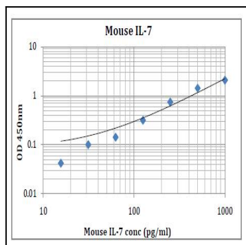
Figure-1: Mouse IL-7 Standard Curve .
