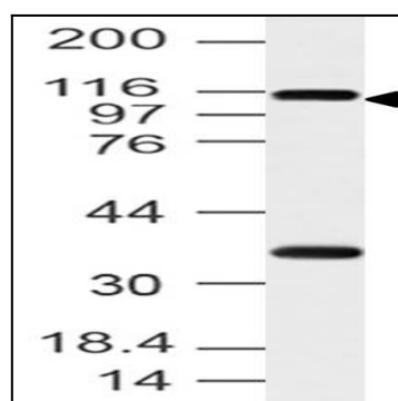
Figure-1: Western blot analysis of FMNL3. Anti-FMNL3 antibody (11-10010) was used at 4 µg/ml on h Stomach lysate.
