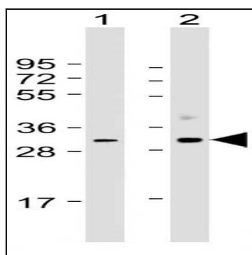
Figure 1: All lanes : Anti-CDK1 Antibody (10-6630) at 1:500-1:1000 dilution with Lane 1: Jurkat whole cell lysate, Lane 2: Hela whole cell lysates/proteins at 20 µg per lane. Secondary Goat Anti-mouse IgG, (H+L), Peroxidase conjugated at 1/10000 dilution. Predicted band size : 34 kDa.
