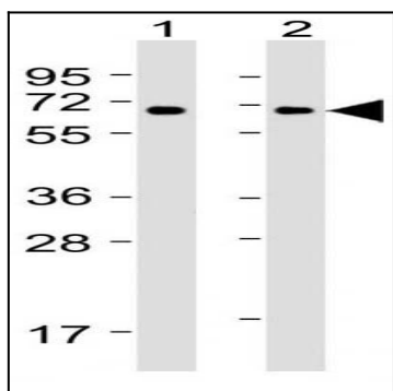
Figure 3: All lanes: Anti-ZAP70 Antibody (10-6628) at 1:4000 dilution with Lane 1: Jurkat whole cell lysates, Lane 2: MOLT-4 whole cell lysates /proteins at 20 µg per lane. Secondary Goat Anti-mouse IgG, (H+L), Peroxidase conjugated at 1/10000 dilution. Predicted band size: 70 kDa.
