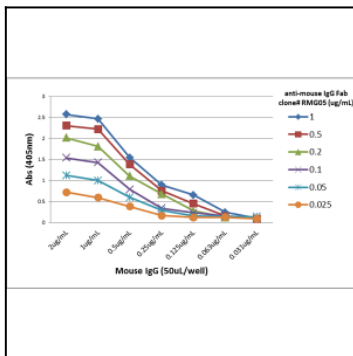
Figure 2: A titer ELISA of mouse IgG. The plate was coated with different amounts of mouse IgG. A serial dilution of Clone: RMG05 was used as the primary antibody. An alkaline phosphatase conjugated anti-goat IgG as the secondary antibody.
