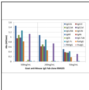
Figure 1: ELISA of mouse immunoglobulins shows Clone: RMG05 reacts to the Fab region of mouse IgG1, IgG2a, IgG2b, and IgG3; no cross reactivity with IgM, IgA, IgE, human IgG, rat IgG, and rabbit IgG. The plate was coated with 50 ng/well of different immunoglobulins. 500 ng/ml, 200 ng/ml, or 50 ng/ml of Clone: RMG05 was used as the primary antibody. An alkaline phosphatase conjugated anti-goat IgG as the secondary antibody.
