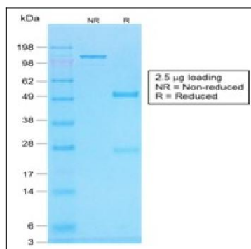
Figure 3: SDS-PAGE Analysis of Purified Histone H1 Mouse Recombinant Monoclonal Antibody (r1415-1).
