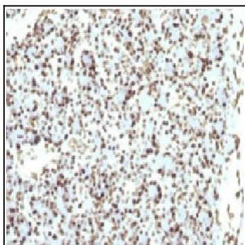
Figure 2: Formalin-fixed, paraffin-embedded Rat Pancreas stained with Histone H1 Mouse Recombinant Monoclonal Antibody (r1415-1).
