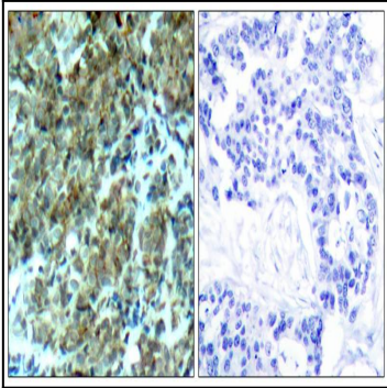
Figure 2: Immunohistochemical analysis of paraffin-embedded human breast carcinoma tissue using Cortactin(Ab-466) Antibody 35-1597 (left) or the same antibody preincubated with blocking peptide(right).
