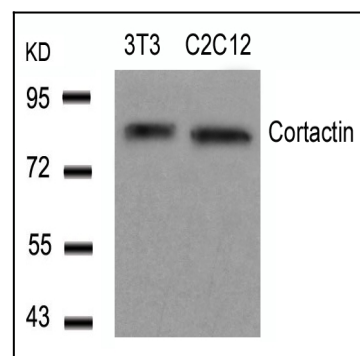
Figure 1: Western blot analysis of extracts from 3T3 and C2C12 cells using Cortactin(Ab-466) Antibody 35-1597 .
