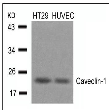
Figure 1: Western blot analysis of extracts from HT29 and HUVEC cells using Caveolin-1 (Ab-14) Antibody 35-1464 .
