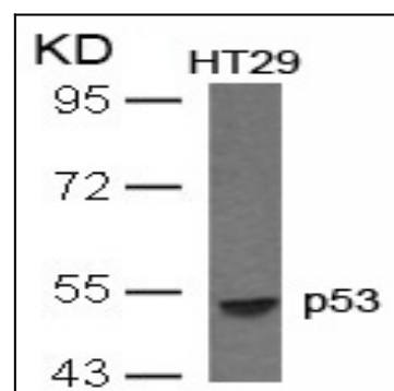
Figure 1: Western blot analysis of extracts from HT29 cells using p53(Ab-33) Antibody 35-1441 .
