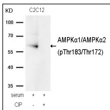
Figure 2: Western blot analysis of extracts from C2C12 cells, treated with serum or calf intestinal phosphatase (CIP), using AMPK \alpha 1/AMPK \alpha 2(Phospho-Thr174/Thr172) Antibody 35-1173.
