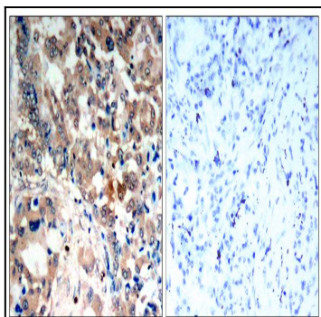
Figure 1: Immunohistochemical analysis of paraffin-embedded human lung carcinoma tissue, using AMPK \alpha 1/AMPK \alpha 2(Phospho-Thr174/Thr172) Antibody (35-1173).
