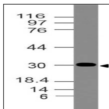
Fig-1: Western blot analysis of NKx2.2 . Anti-NKx2.2 antibody (11-7578) was used at 2 µg/ml on h Brain lysate.
