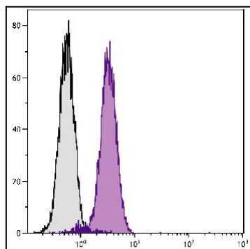
Figure 1: T cell leukemia cell line Jurkat was intracellularly stained with Mouse Anti-Human Bcl-xL-FITC .
