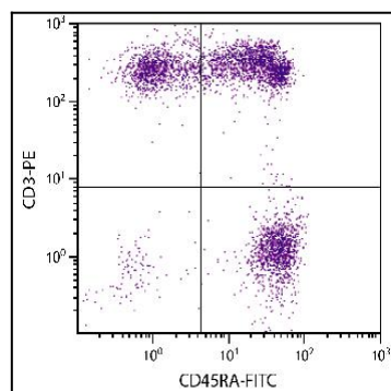
Figure 1: Human peripheral blood lymphocytes were stained with Mouse Anti-Human CD45RA-FITC and Mouse Anti-Human CD3-PE .
