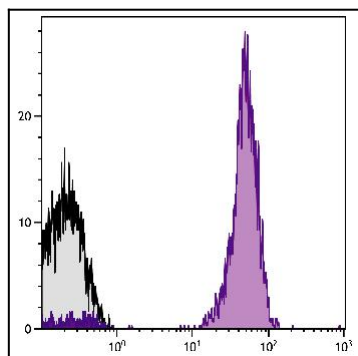
Figure 1: Human peripheral blood lymphocytes were stained with Mouse Anti-Human CD45-PE/CY7 .
