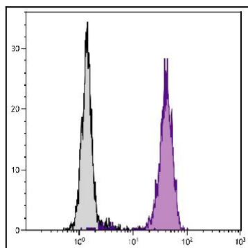
Figure 1: Human granulocytes were stained with Mouse Anti-Human CD16-Biotin followed by Streptavidin-FITC .
