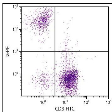
Figure 1: Chicken peripheral blood mononuclear cells were stained with Mouse Anti-Chicken Ia-PE and Mouse Anti-Chicken CD3-FITC .
