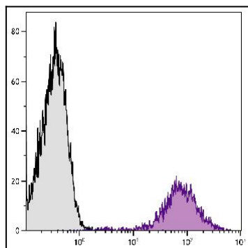
Figure 1: Con-A stimulated BALB/c mouse splenocytes were stained with Rat Anti-Mouse Ly-6A/E-PE/CY5.5 .
