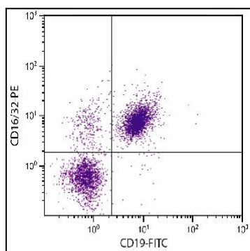
Figure 1: BALB/c mouse splenocytes were stained with Rat Anti-Mouse CD16/32-PE and Rat Anti-Mouse CD19-FITC .
