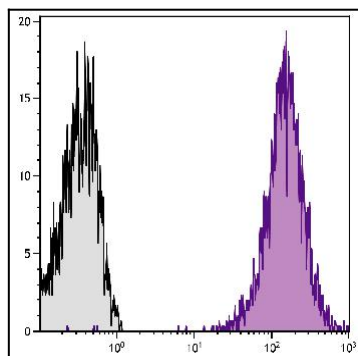
Figure 1: C57BL/6 mouse cytotoxic T lymphocyte cell line CTLL-2 was stained with Rat Anti-Mouse CD25-PE/CY7 .
