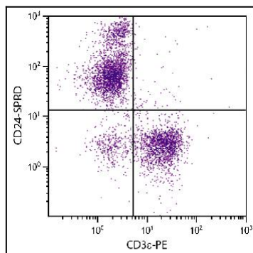
Figure 1: BALB/c mouse splenocytes were stained with Rat Anti-Mouse CD24-SPRD and Rat Anti-Mouse CD3e-PE .
