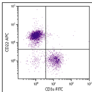
Fig 1: BALB/c mouse splenocytes were stained with Rat Anti-Mouse CD22-APC and Rat Anti-Mouse CD3 \epsilon -FITC
