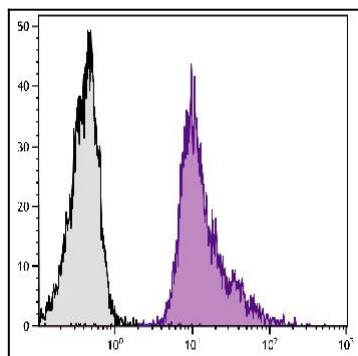
Figure 1: BALB/c mouse splenocytes were stained with Rat Anti-Mouse CD18-Biotin followed by Streptavidin-FITC .
