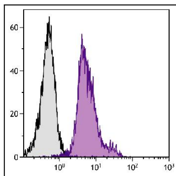
Figure 1: BALB/c mouse splenocytes were stained with Rat Anti-Mouse CD11a-FITC .
